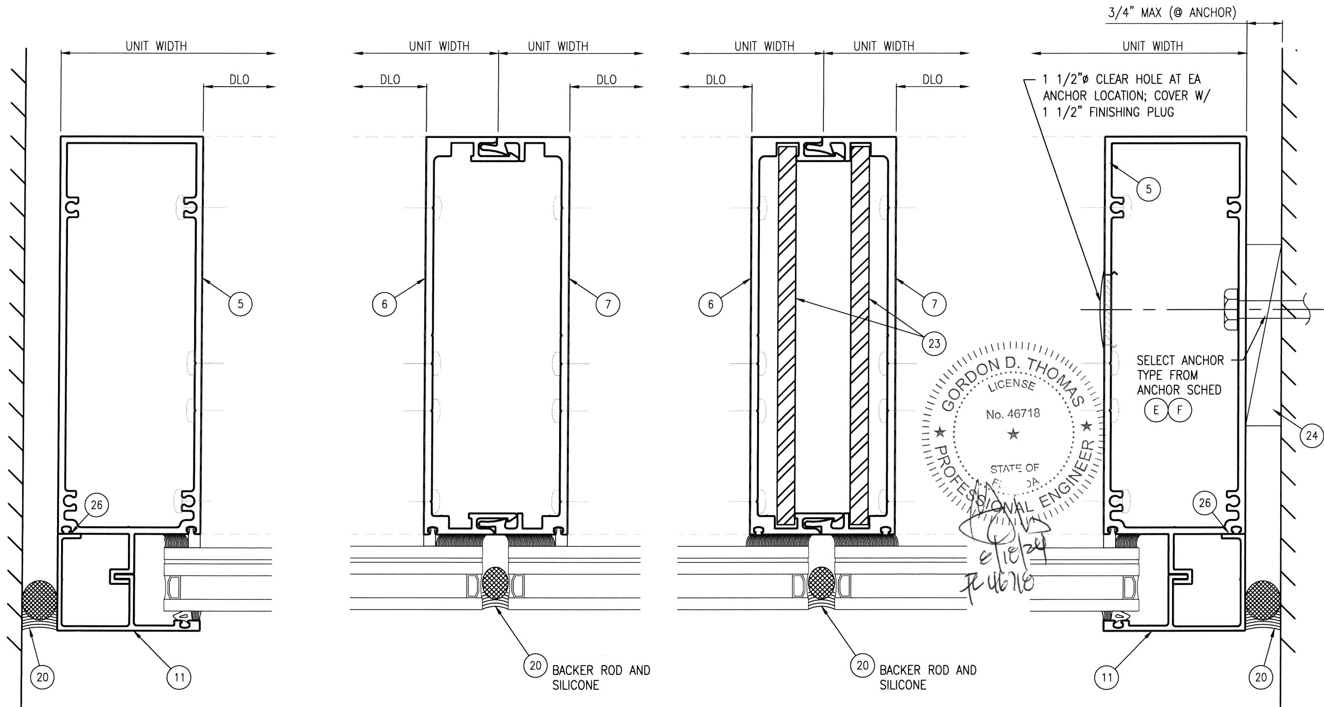
1 UNANCHORED JAMB Glazing condition G2 Scale: 6" = 1'-0"
