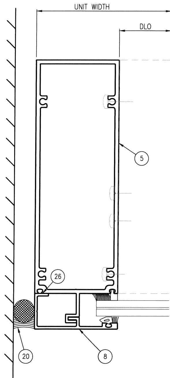
1 UNANCHORED JAMB Glazing condition G1 Scale: 6" = 1'-0"
