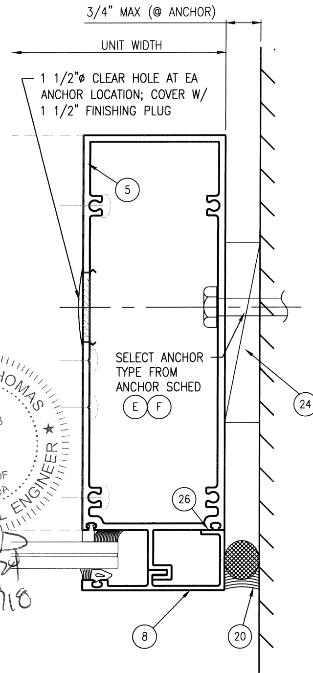
4 ANCHORED JAMB Glazing condition G1 Scale: 6" = 1'-0"
